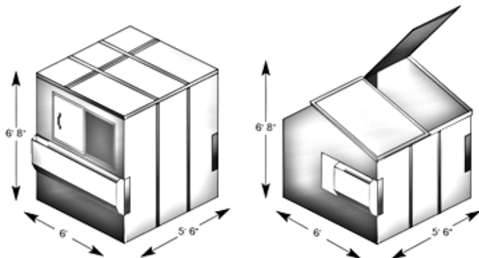
8 YARD FLAT AND SLANTED
